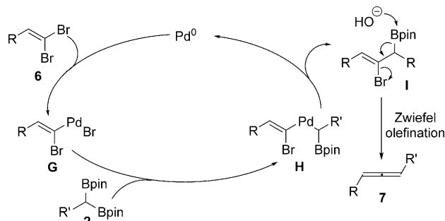
Scheme 8. Proposed reaction mechanism.
