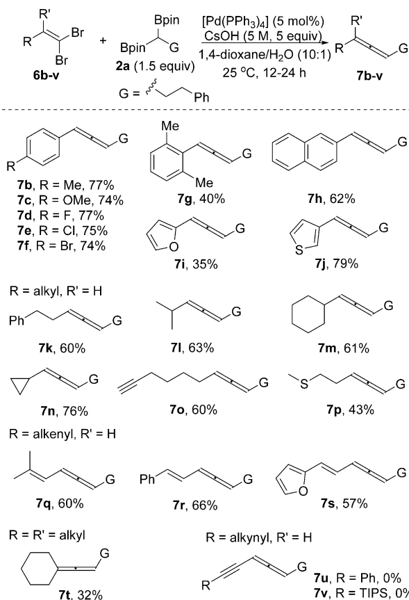
Scheme 5. Substrate scope of 1,1-dibromoalkenes. Reaction conditions: 6 (0.5 mmol), 2a (0.75 mmol), [Pd(PPh 3 ) 4 ] (0.025 mmol), CsOH (5 M, 500 \mu L), 1,4-dioxane (5 mL). Products were isolated by silica gel chromatography. TIPS = triisopropylsilyl.
