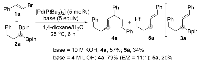
Scheme 2. Reactions of 1,1-diboronates with vinyl bromide. Reaction conditions: 1a (0.4 mmol), 2a (0.3 mmol), [Pd(PtBu 3 ) 2 ] (5 mol%), base, 1,4-dioxane (2 mL). The products were isolated by silica gel chromatography. The E/Z ratio was determined by 1 H NMR analysis of the final product.
